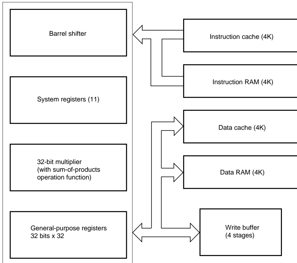
Figure 1-1. Internal Configuration
